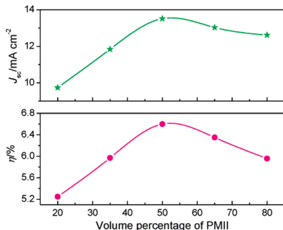
Figure 6. Dependence of photocurrent density and power conversion efficiency of devices under the AM 1.5 full sunlight ( 100 \text{ mW cm}^{-2} ) on the volume percentage of PMII. The iodine concentration is kept at 0.2 M.
