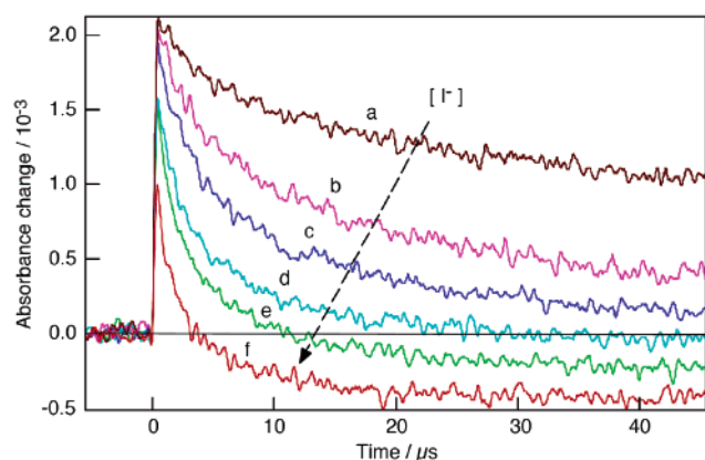
Figure 7. Transient absorbance at 630 nm of dye-sensitized transparent \text{TiO}_2 films in binary mixtures of PMII and EMITCM. The iodide concentration was increased from 0 to 5.8 M by raising the PMII volume percentage: (a) 0%; (b) 5%; (c) 11%; (d) 23%; (e) 45%; (f) 100%.
